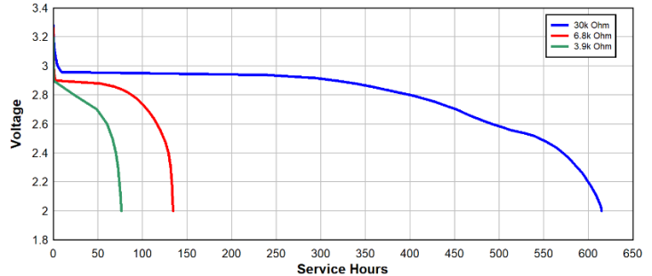
Continuous Discharge at Various Loads
