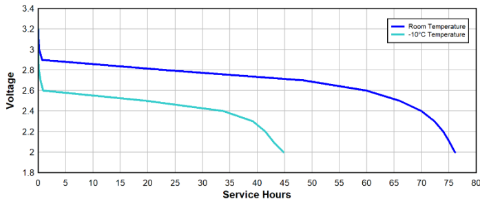
Temperature Performance 3.9k Ohm Continuous to 2V
